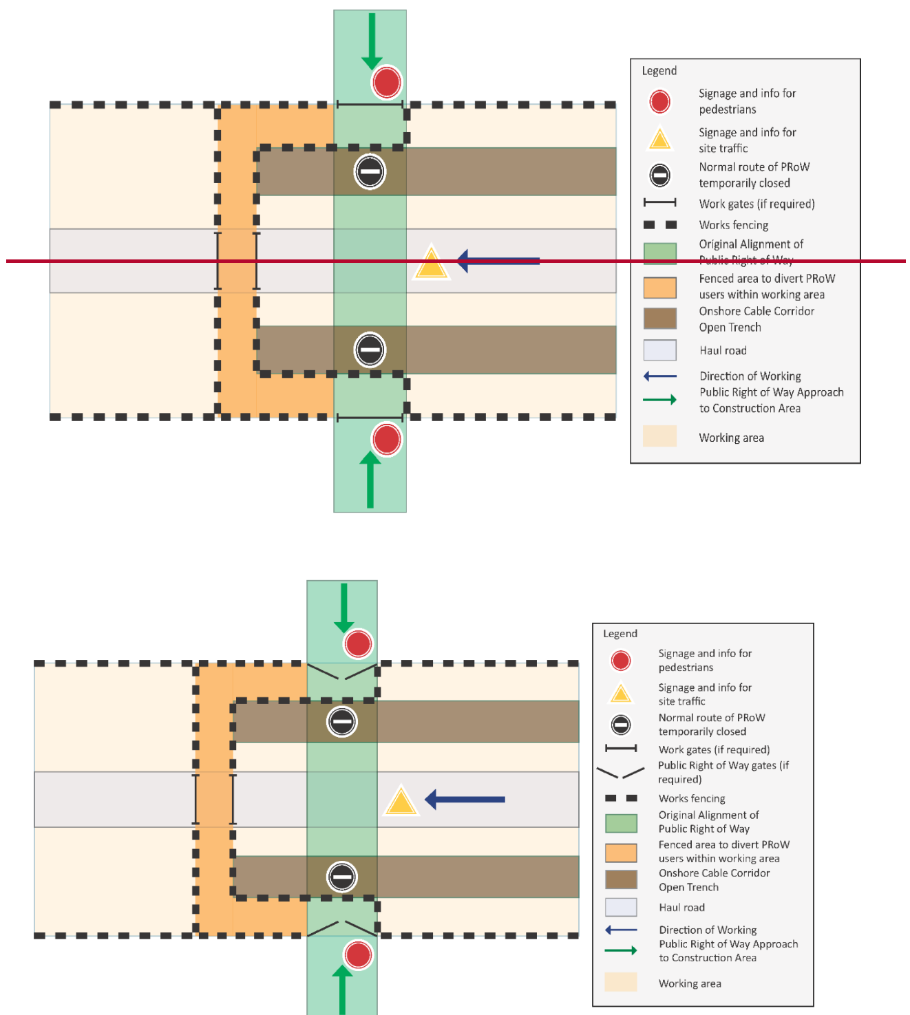
Figure 1.3: Illustrative diagram of temporary diversion of a PRoW
